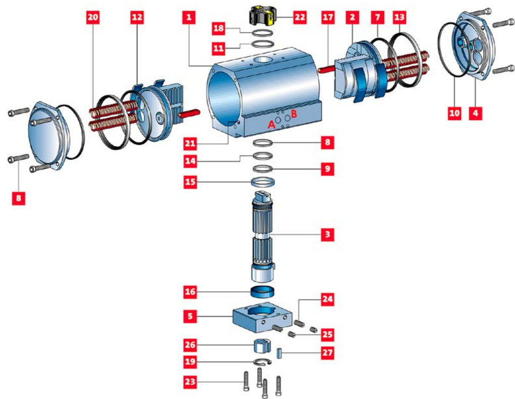
Nomenclature Type "E / C" "E/C" Type Components
