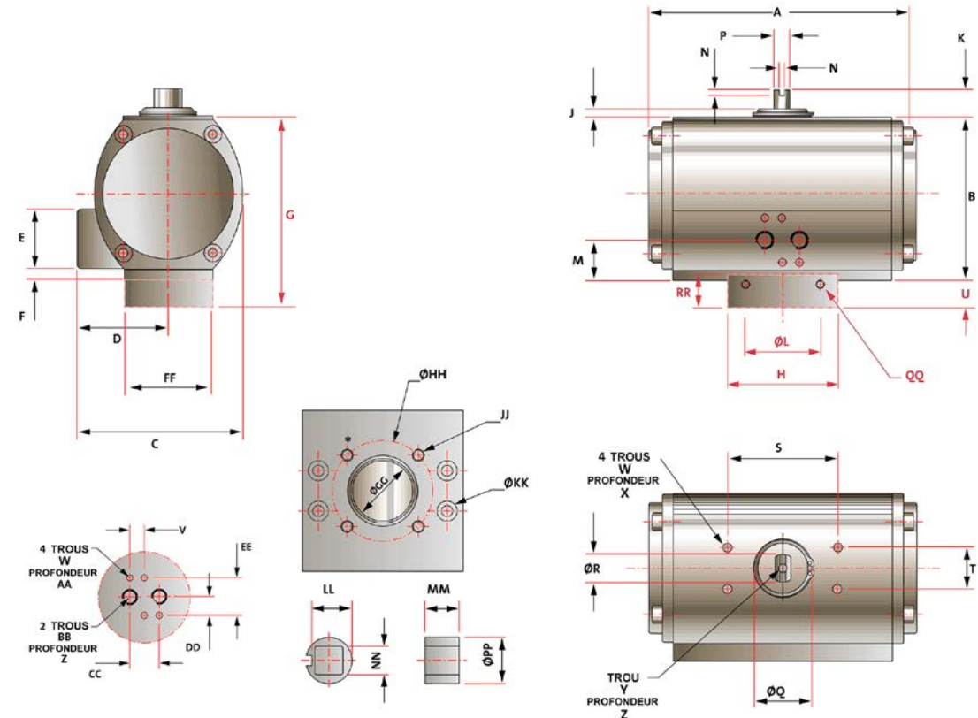
Dimensions actionneur type "E" Overall dimensions "E" type
