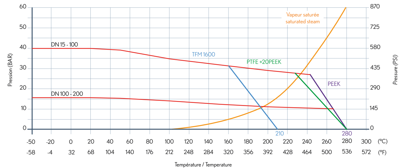
Courbes Pression/Température / Pressure/Temperature diagrams
